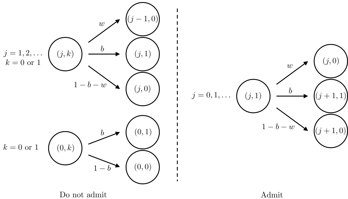
Figure 3.7: Possible state transitions for admission control problem. Note that not admitting a waiting job results in the same transitions as when no job arrives.
